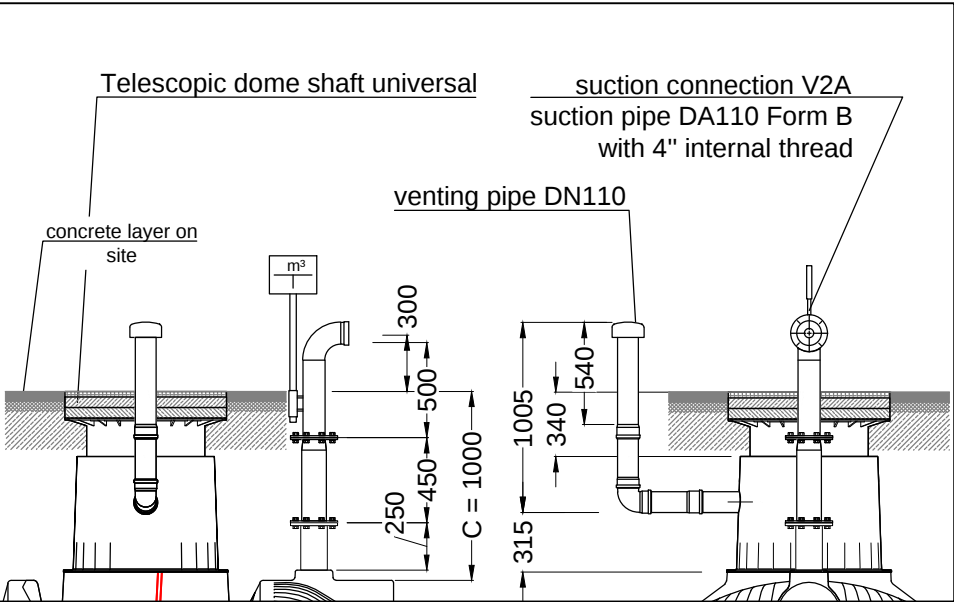
Detail A1, earthcovering = 1000mm
