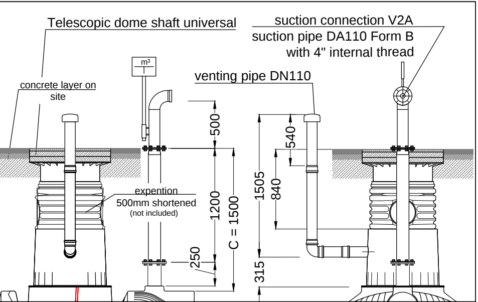
Detail A3, earthcovering = 1500mm
