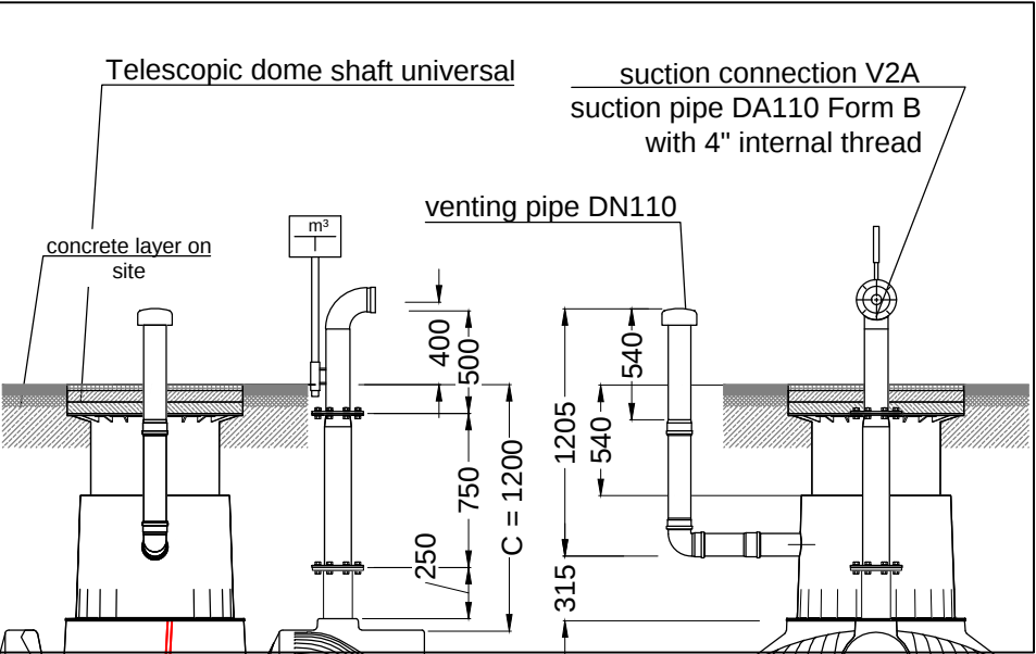
Detail A2, earthcovering = 1200mm
