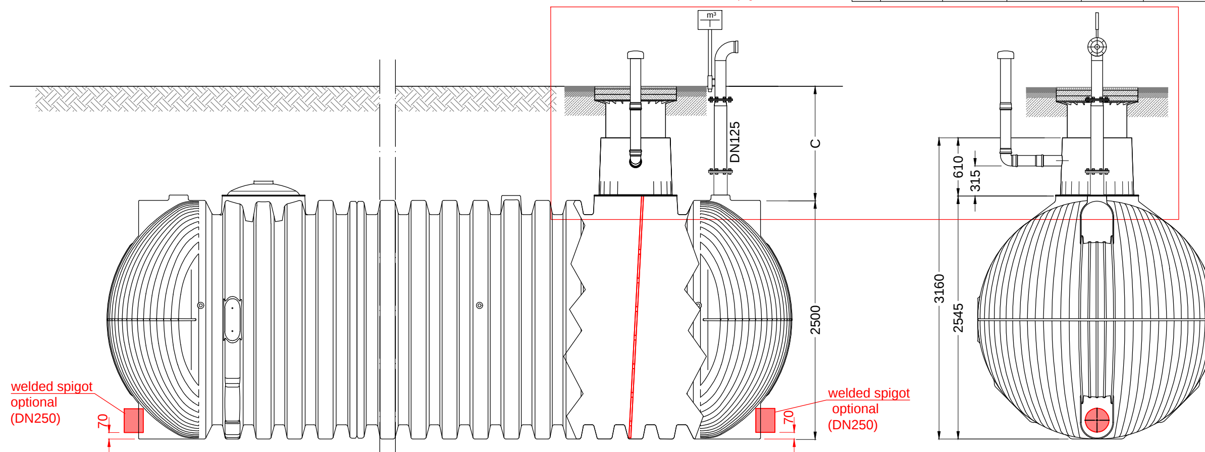
Detail A1-A3 see page 02
