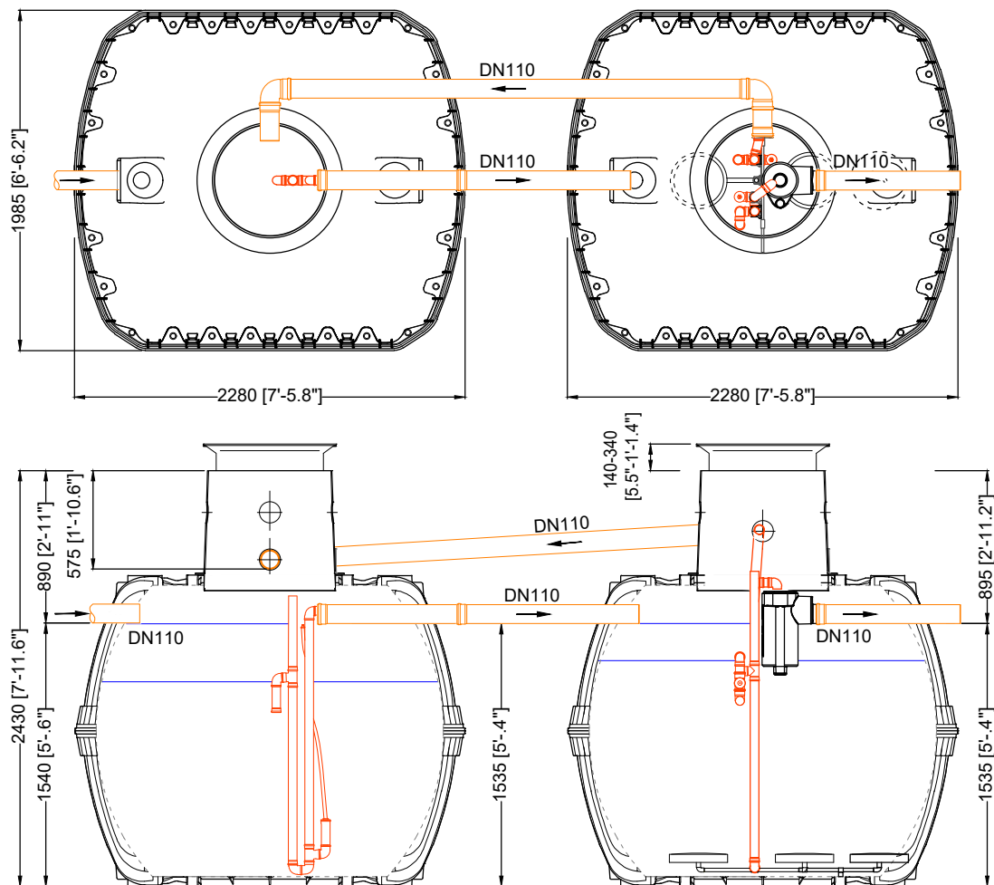
sludge storage/ buffer
